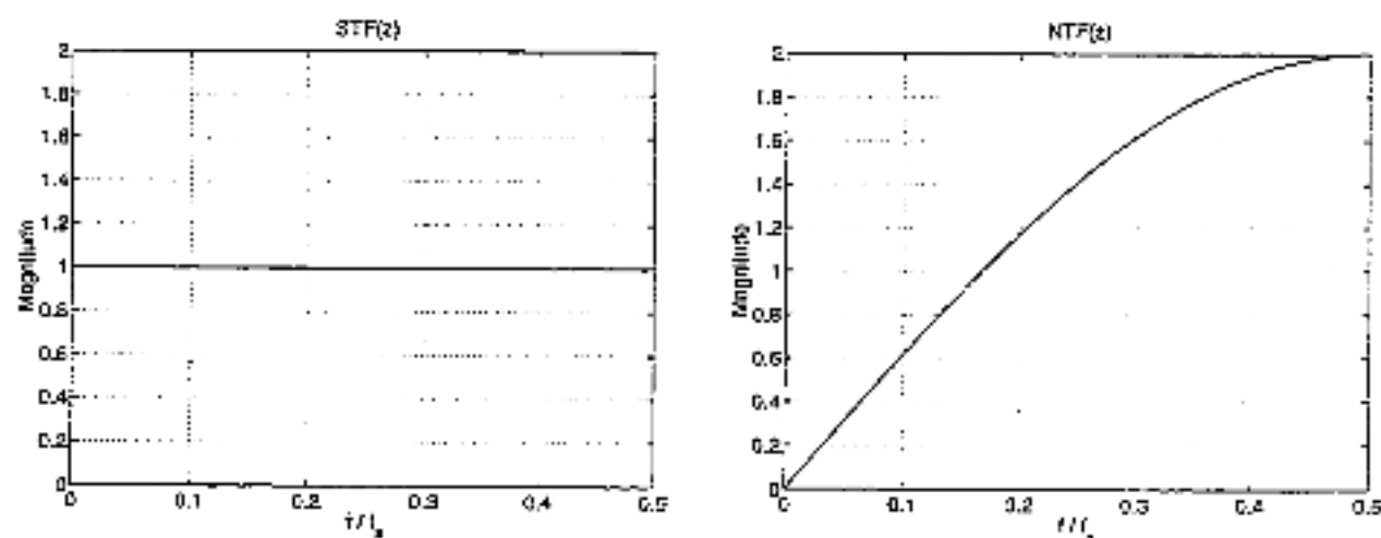
Figure 2.3: \text{STF}(z) and \text{NTF}(z) for circuit of Example 2.1.
