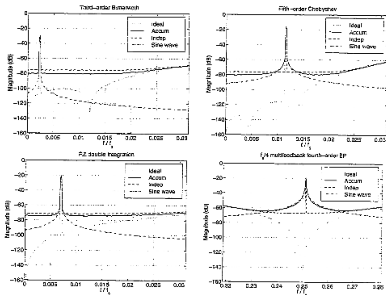
Figure 5.9: Comparison of \Delta\Sigma M spectra for independent and accumulated jitter, including spectrum of single tone at output of jittered S/H.
