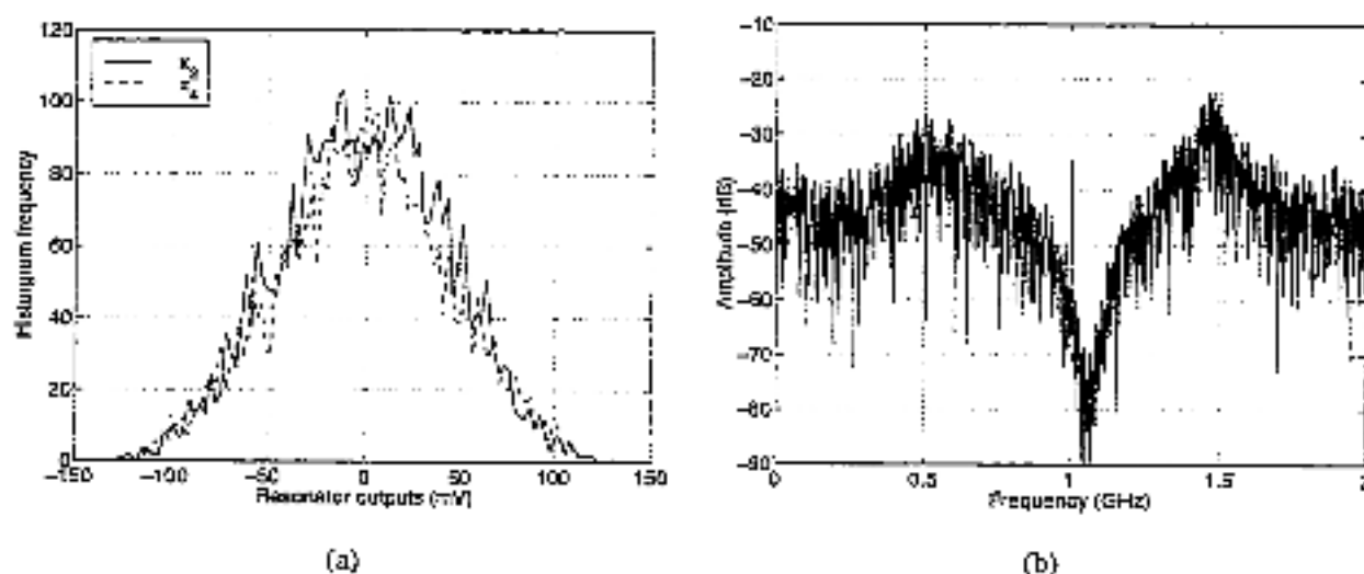
Figure 7.58: Scaled DAC currents k_{m2} \approx k_{m4} = 1.8\text{mA} : (a) resonator output histograms, (b) output spectrum.
