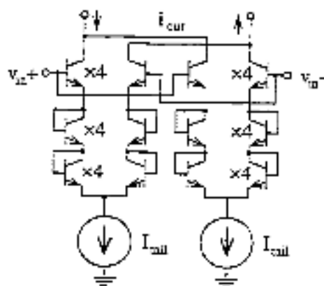
Figure 7.12: Actual transconductance topology used.
