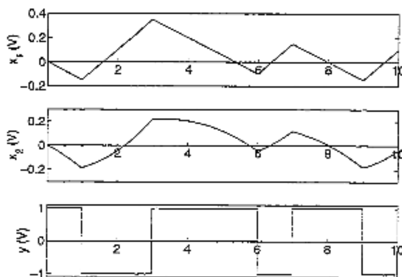
Figure 3.1: Typical integrator output and quantizer waveforms.
