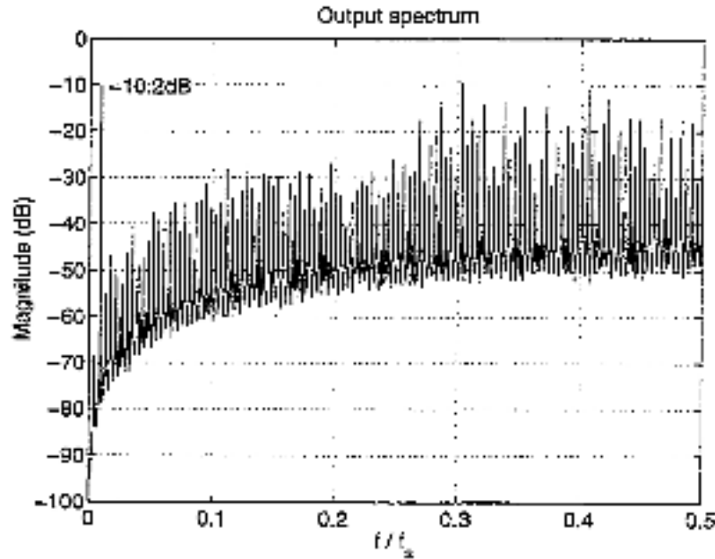
Figure 2.4: Simulated output bit stream power spectrum.
