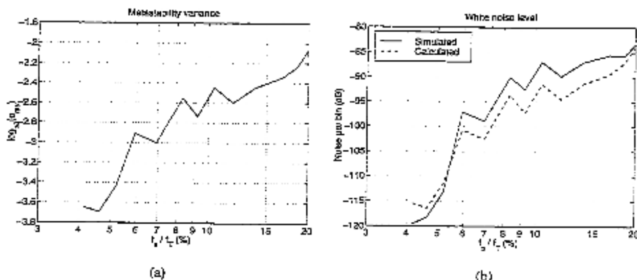
Figure 6.23: Effect of increasing f_s on (a) \sigma_{mss} , (b) calculated and simulated noise level.
