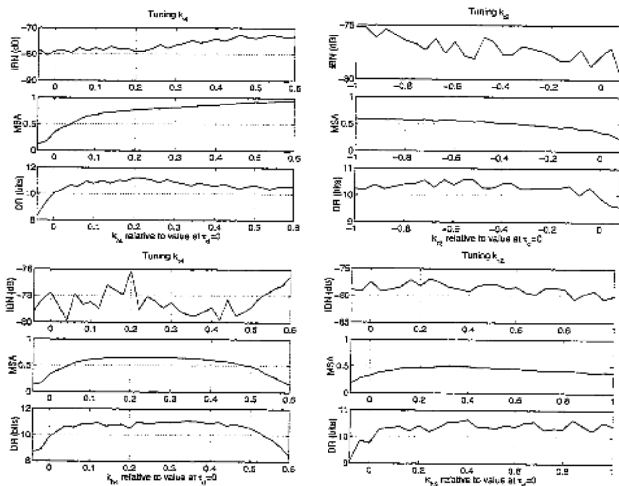
Figure 4.22: Fourth-order f_s/4 BP CT \Delta\Sigma M performance at p_d = 35\% delay with feedback coefficient tuning.
