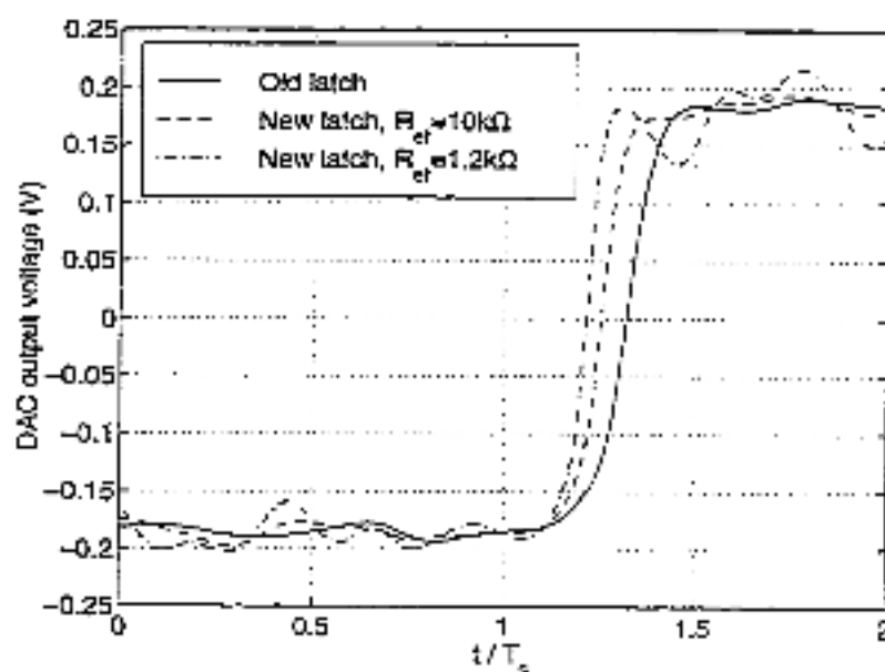
Figure 7.53: Dynamic DAC output voltage.
