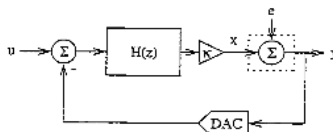
Figure 4.6: Linearized \Delta\Sigma\text{M} with one-bit quantizer arbitrary gain \kappa .
