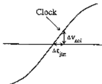
Figure 7.47: Clock jitter caused by circuit noise.
