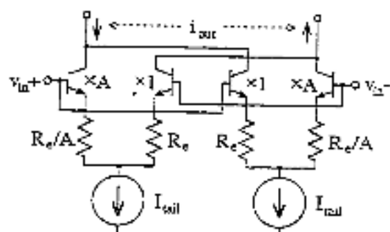
Figure 7.10: Multi-tanh circuit.
