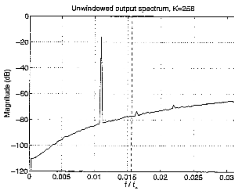
Figure 2.11: Unwindowed averaged periodogram near dc.
