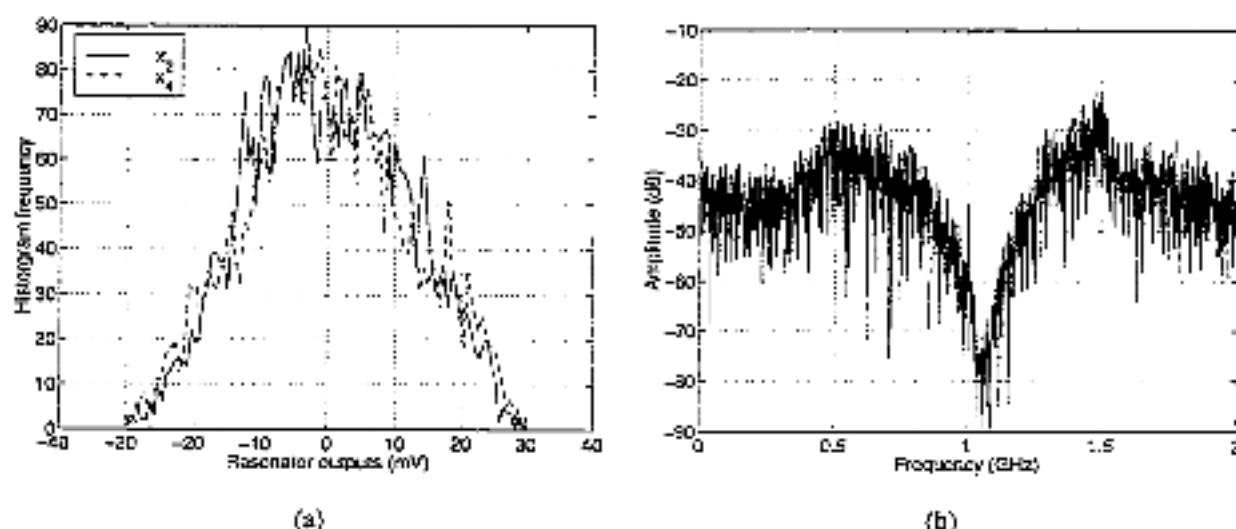
Figure 7.57: Scaled DAC currents k_{N1} = k_{N4} = 500\mu\text{A} : (a) resonator output histograms, (b) output spectrum.
