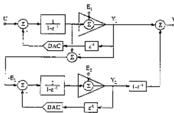
Figure 2.8: A multistage \Delta\Sigma .
