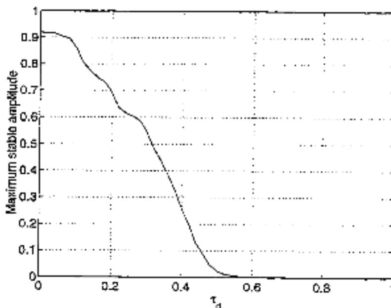
Figure 4.9: Maximum stable amplitude for double integration CT \Delta\Sigma .
