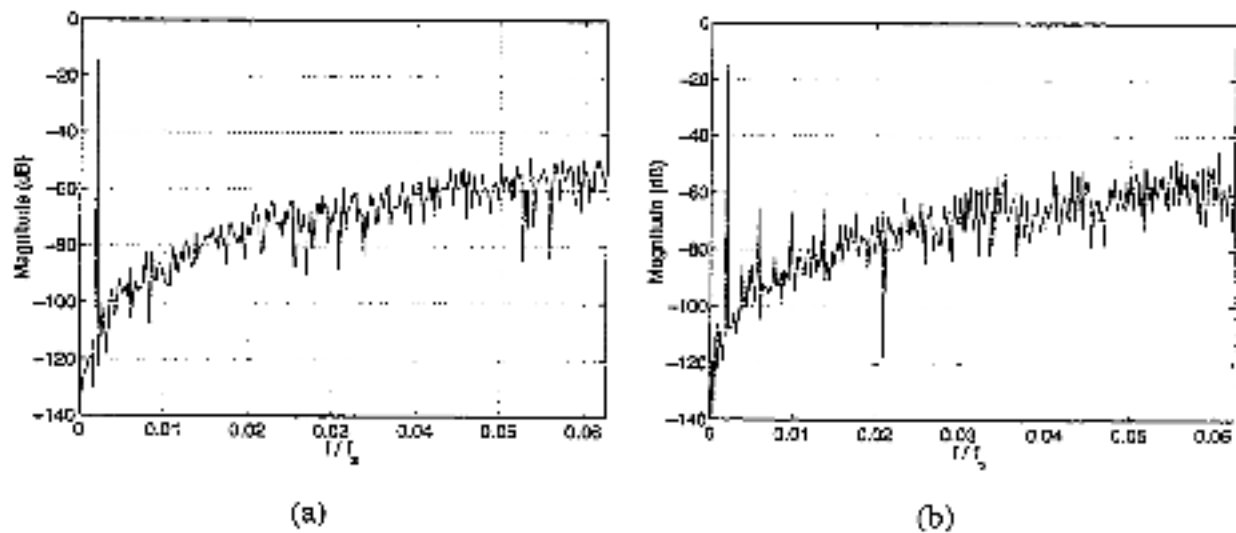
Figure 3.2: Output spectra using op amps with (a) no slow-rate limiting, (b) slow-rate limiting.
