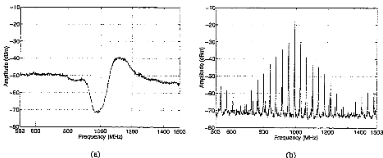
Figure 7.35: Oscillation in output spectrum: (a) V_Q = 3.31V , (b) V_Q = 3.33V .
