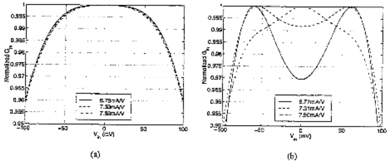
Figure 7.15: Linearity for emitter diodes vs. emitter resistors: (a) A = 4 , D = 3 , (b) A = 8 . R_2 = 100\Omega .
