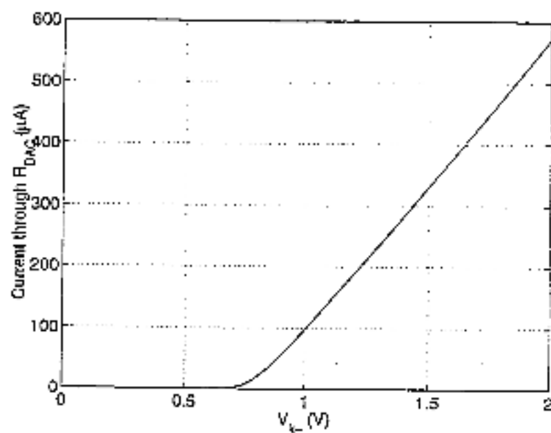
Figure B.4: DAC current vs. control voltage.
