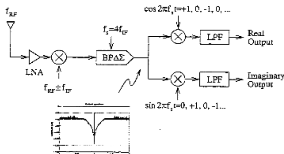
Figure 2.7: Typical radio receiver application for a band pass \Delta\Sigma M.
