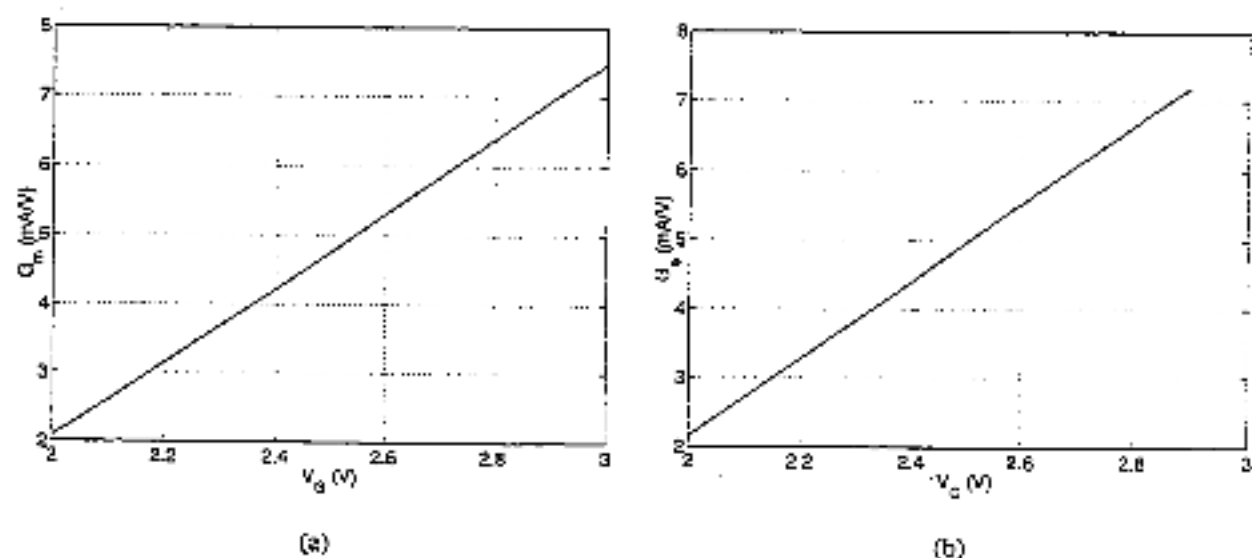
Figure B.2: (a) G_S against V_G , (b) G_D against V_G .
