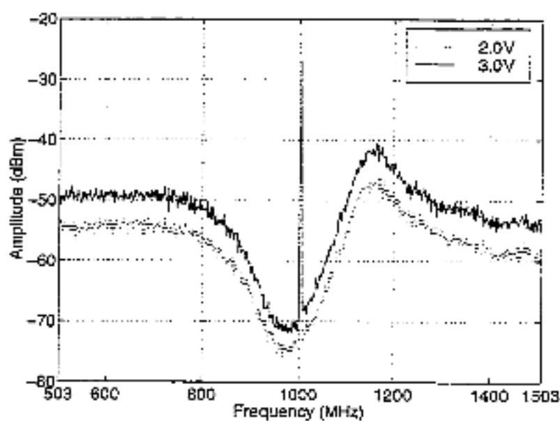
Figure 7.41: Varying V_{BDS} .
